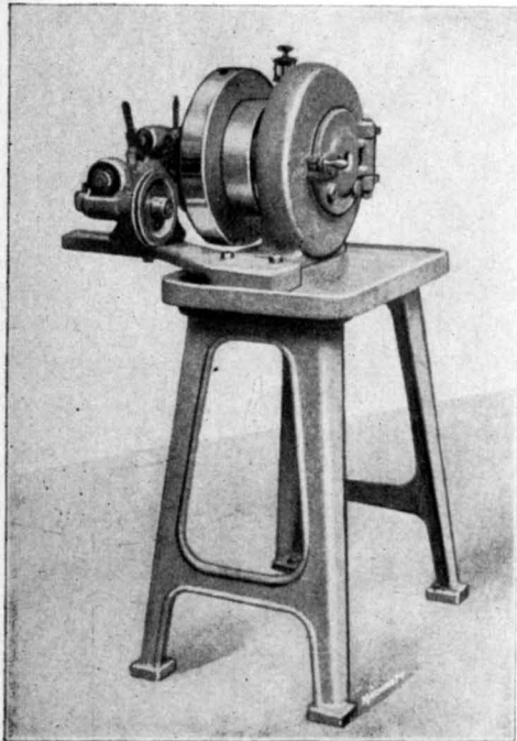
Fig. 4. Langelier Swaging Machine
